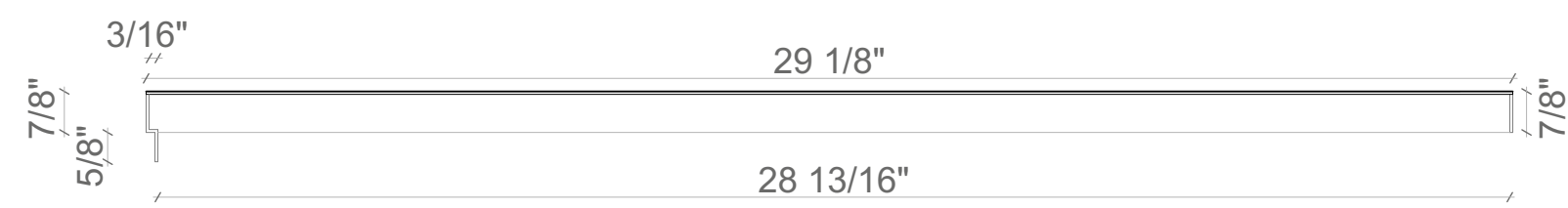
1 SIDE PLATE PIECE (TOP VIEW)
