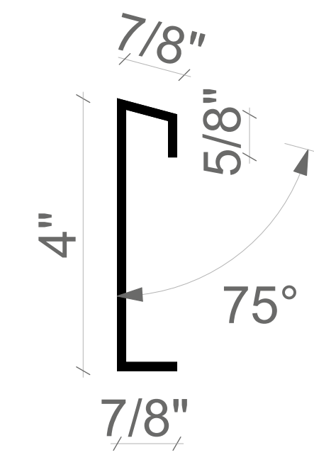
2 BACK PIECE, DOOR PARTS (BUILDING SECCION)
