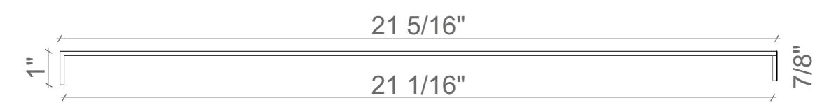
1 TOP COVER PIECE BIN DOOR PARTS (FRONT VIEW)
