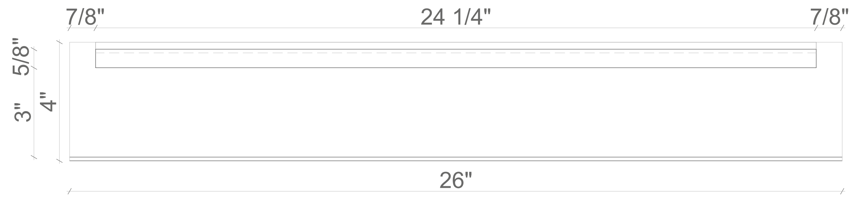
1 BACK PIECE DOOR PARTS (FRONT VIEW)
