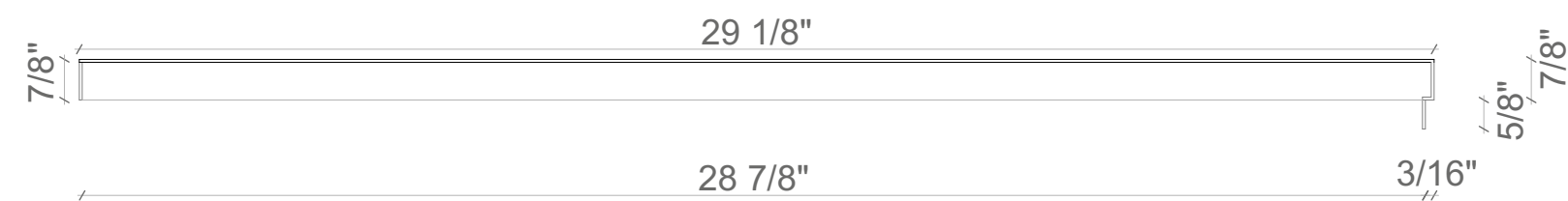
1 SIDE PLATE PIECE (TOP VIEW)
