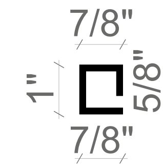
2 SIDE PIECE, DOOR PARTS (BUILDING SECCION)
