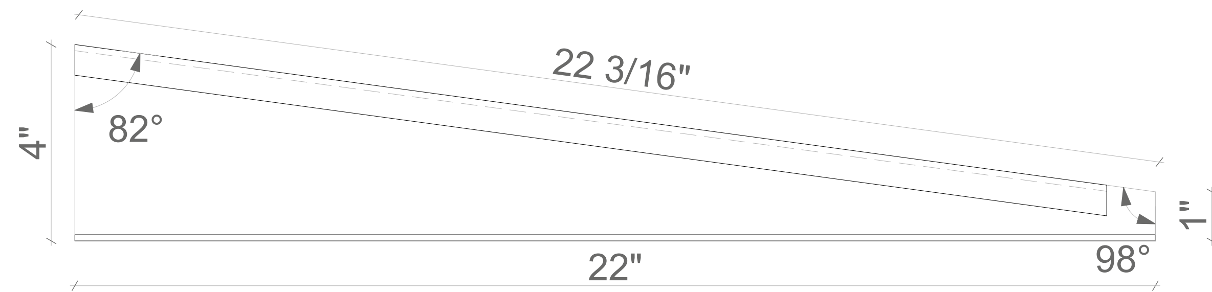
1 SIDE PIECE, DOOR PARTS (SIDE VIEW)
