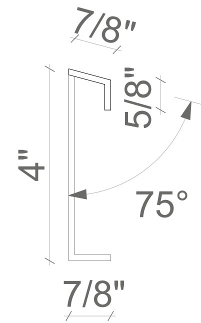
3 BACK PIECE, DOOR PARTS (SIDE VIEW)
