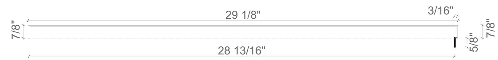
2 SIDE PLATE PIECE (BUILDING SECCION)
