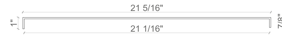
2 TOP COVER PIECE, BIN DOOR PARTS (BUILDING SECCION)
