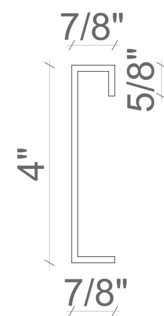
3 SIDE PIECE, DOOR PARTS (FRONT VIEW)
