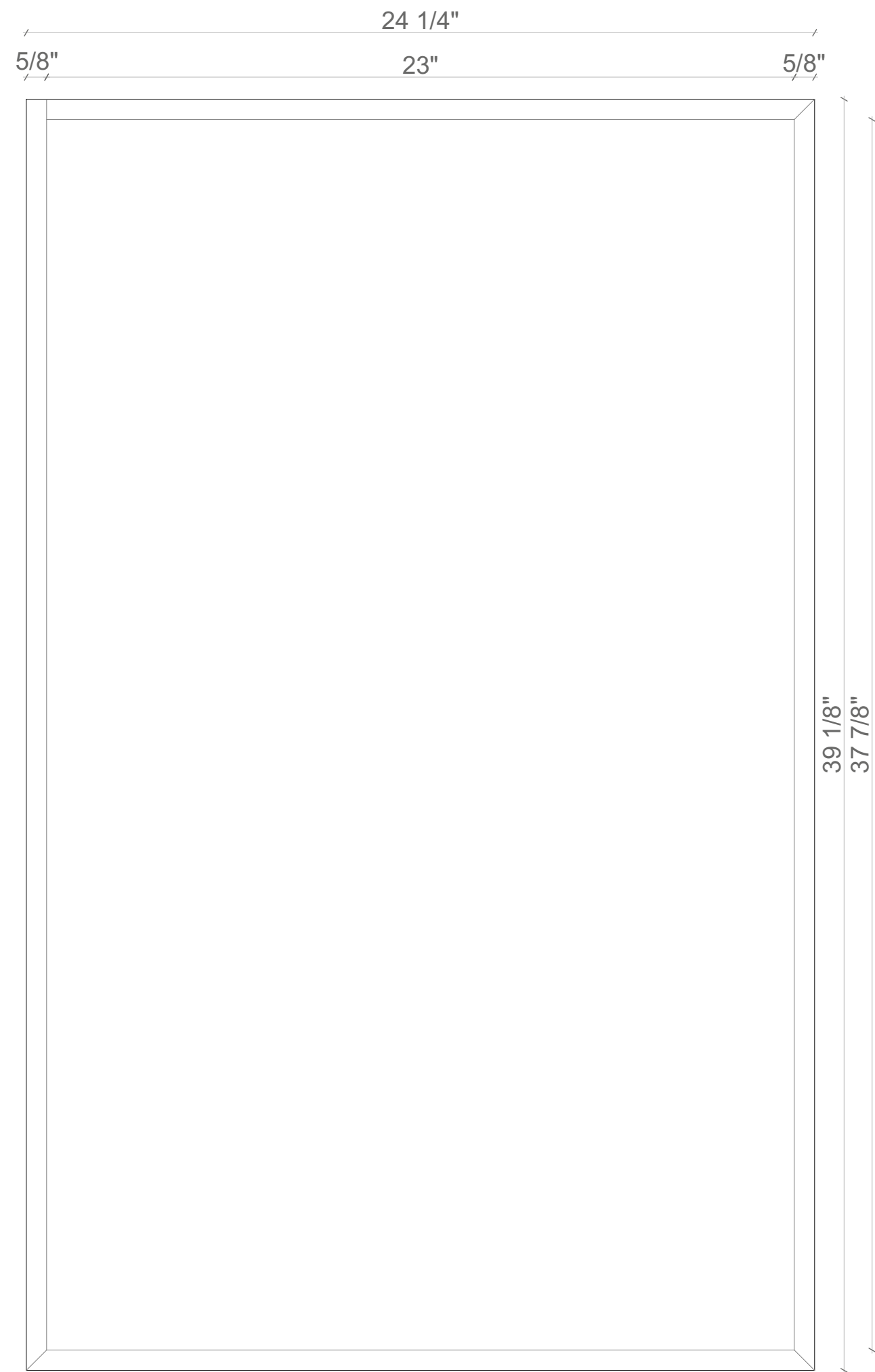
2 GARBAGE DOOR (BACK VIEW)
